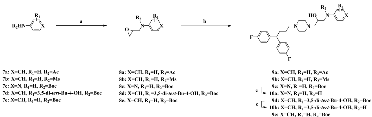
Scheme 3. Reagents and conditions: (a) NaH, epibromohydrin, DMF, room temperature, 34–100%; (b) 1-[4,4-bis(4-fluorophenyl)butyl]piperazine, EtOH, room temperature, 18–74%; (c) \text{HCl}/\text{AcOEt} , room temperature, 50%.
