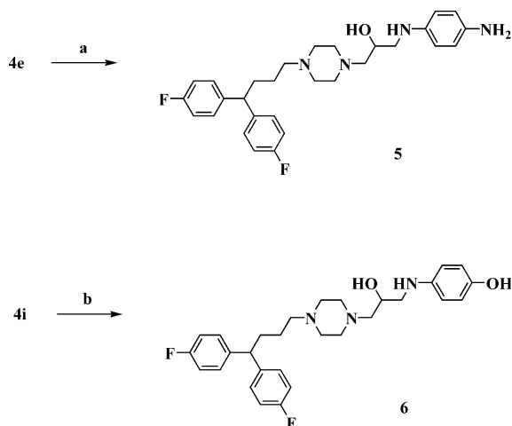
Scheme 2. Reagents and conditions: (a) \text{SnCl}_2 , EtOH, heat, 81%; (b) 10% Pd-black, \text{HCOOH} , MeOH, room temperature, 95%.
