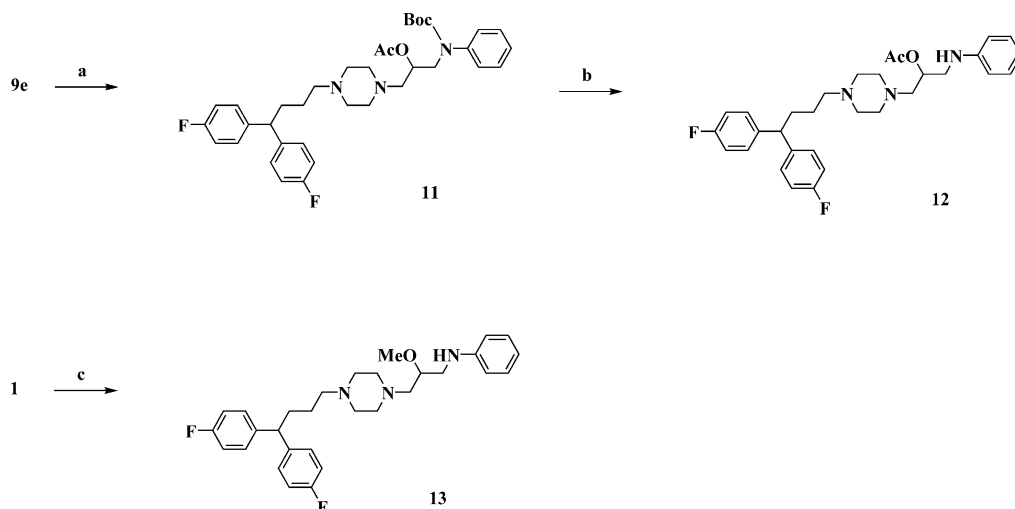
Scheme 4. Reagents and conditions: (a) \text{Ac}_2\text{O} , pyridine, room temperature, 89%; (b) \text{HCl}/\text{AcOEt} , room temperature, 91%; (c) NaH, \text{CH}_3\text{I} , DMF, room temperature, 29%.
