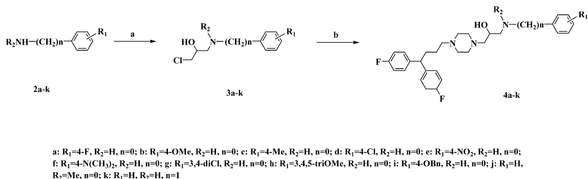
Scheme 1. Reagents and conditions: (a) epichlorohydrin, EtOH, reflux, 42–72%; (b) 1-[4,4-bis(4-fluorophenyl)butyl]piperazine, K 2 CO 3 , KI, EtOH, reflux, 31–78%.
